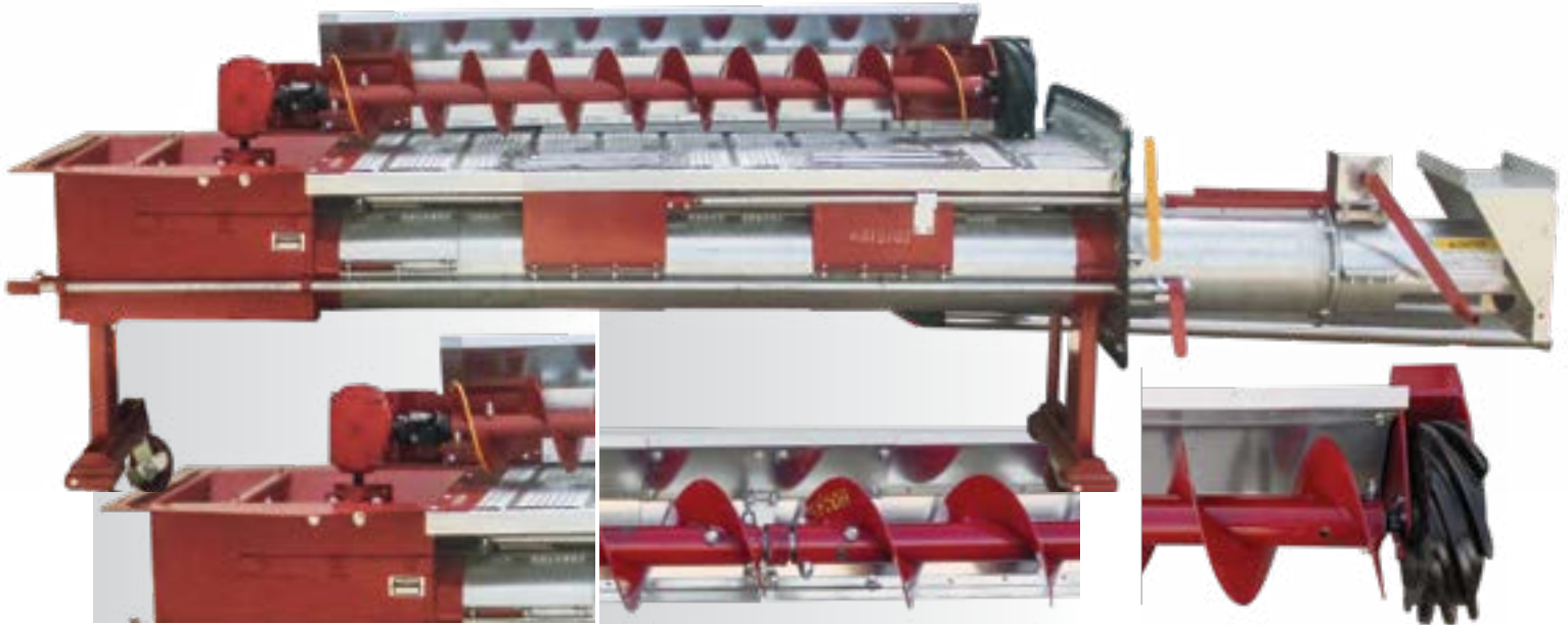
Reduced shaft to get sweep closer to the bin floor
